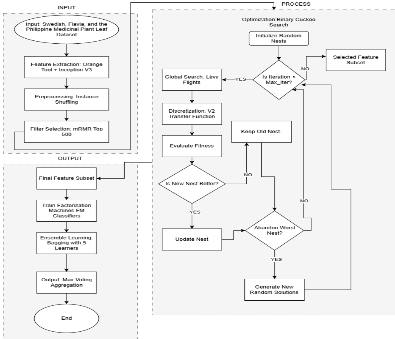
Figure 3. Baseline's Binary Cuckoo Search Architecture
