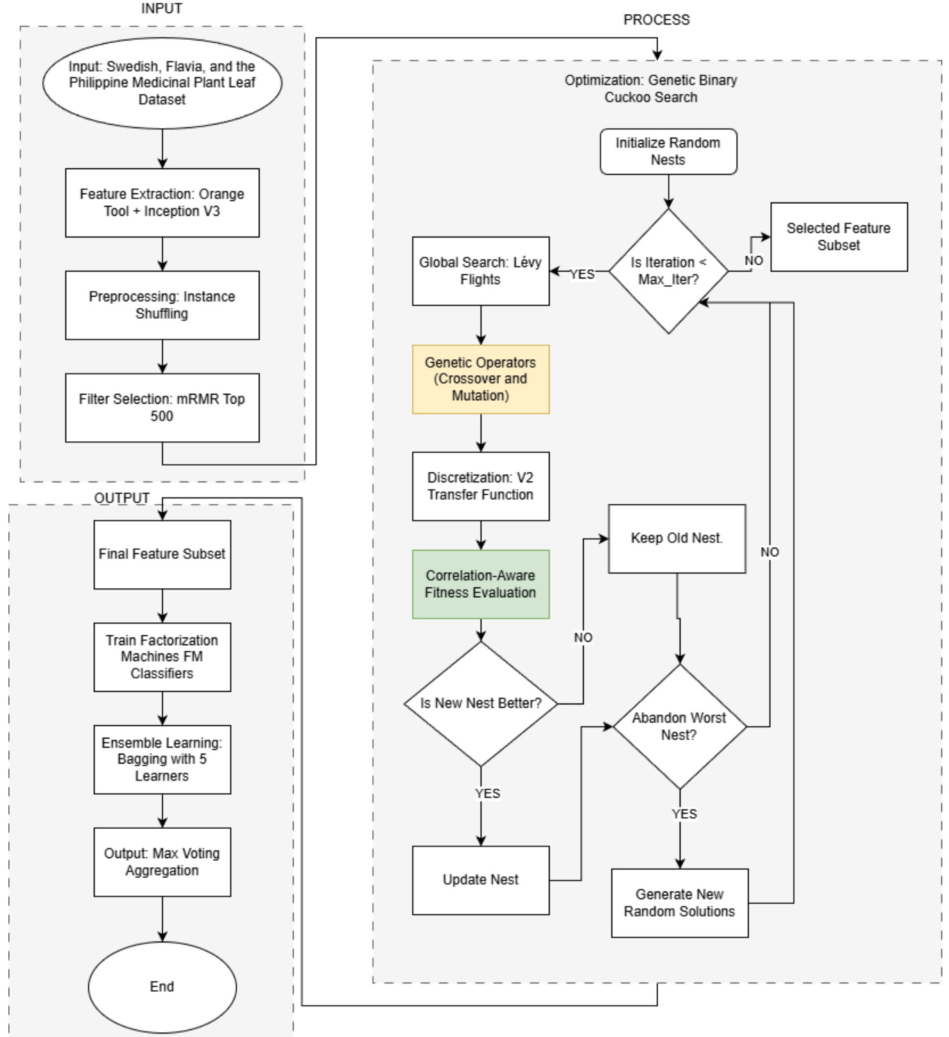
Figure 4. Proposed Genetic Binary Cuckoo Search Architecture
